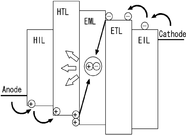
FIG. 2 Related Art
