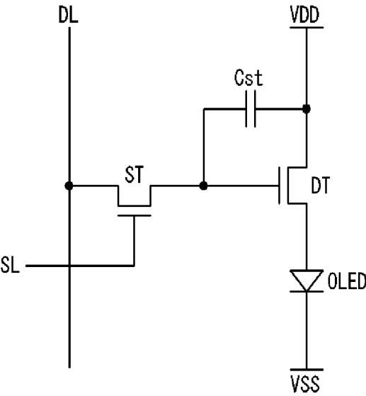
FIG. 2 Related Art
